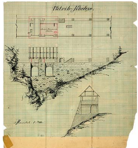
Plan of Putrih's klavže, mid.19th century, Idrija.
